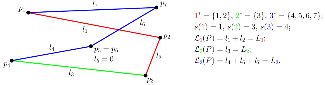
FIGURE 1. A configuration P = (p_1, \dots, p_7) of the necklace \mathbf{N} = ((2, L_1), (1, L_2), (4, L_3))
