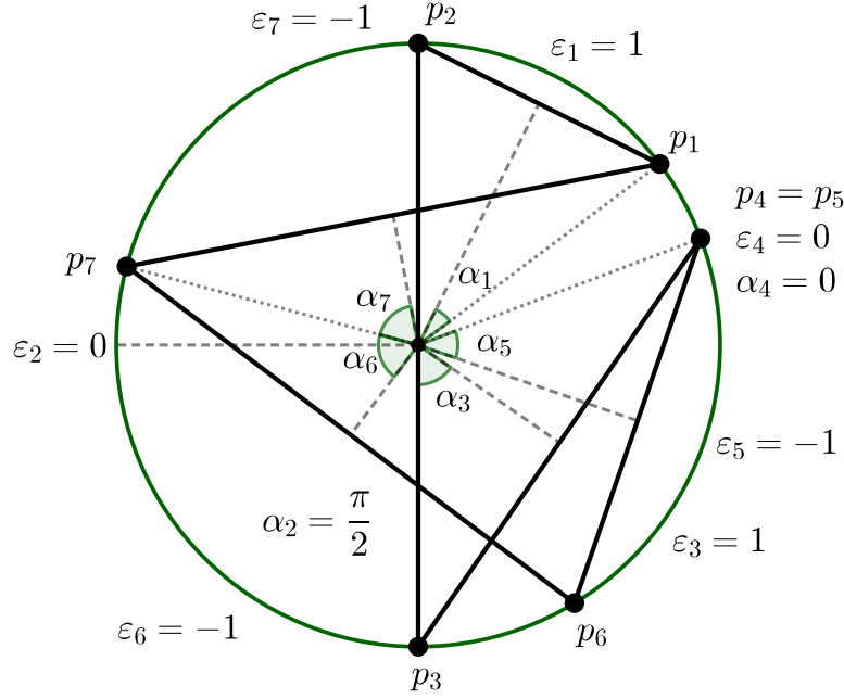
FIGURE 2. Notation for a cyclic polygon
